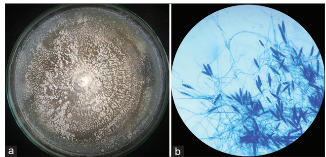
Figure 1: (a) Powdery growth of Nannizzia gypsea on Sabouraud dextrose agar, obverse (b) Nannizzia gypsea showing numerous, thin-walled, spindle-shaped macroconidia (lactophenol cotton blue, 400x).
